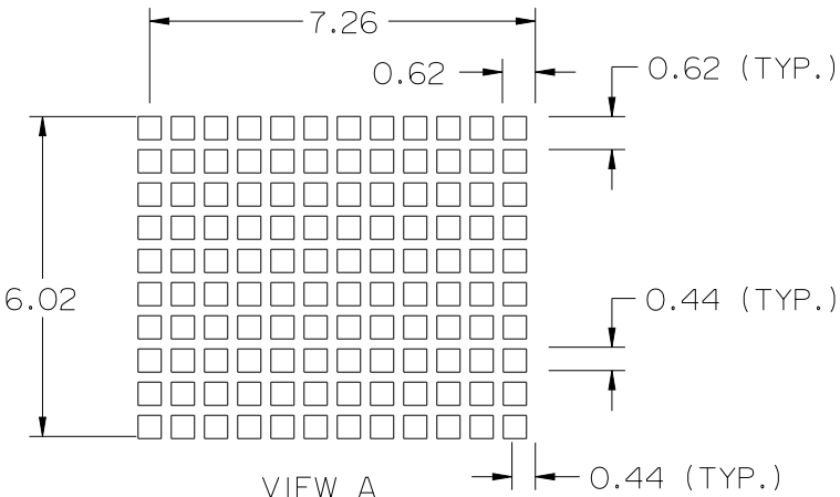
VIEW A TYPICAL VENT PATTERN 0.44 SQ. HOLES (10) VERT. X (12) HORZ.
